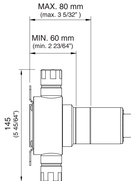
INCLUDED PLUG G 1/2"
