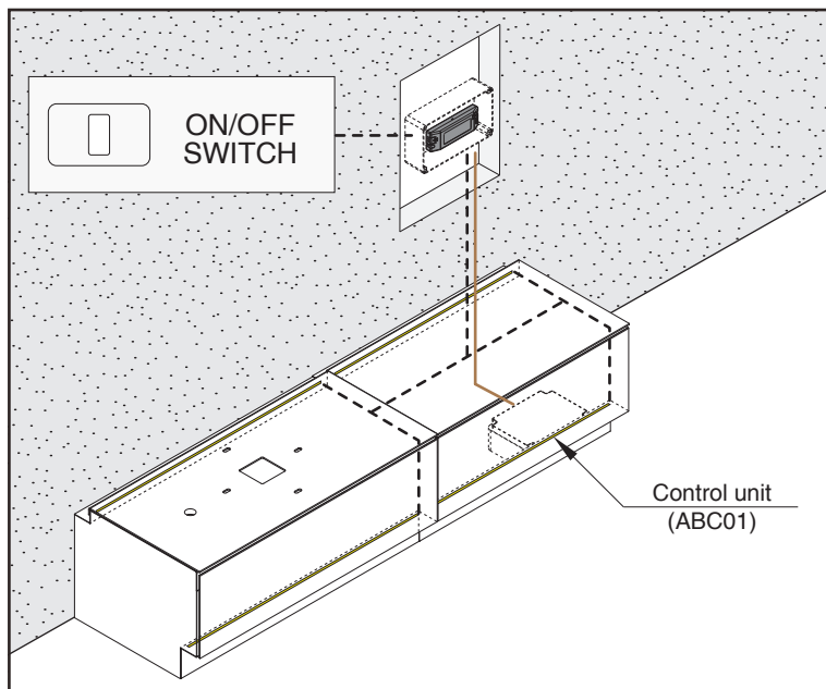
A Switch on/off courtesy lights with remote button
