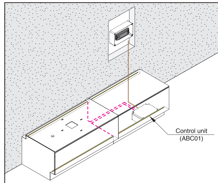
B Switch on/off courtesy lights with presence sensor
