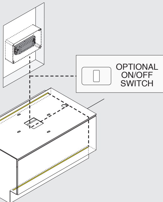
A Switch on/off courtesy lights with remote button
