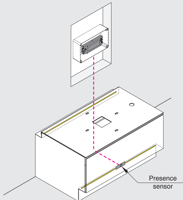
B Switch on/off courtesy lights with presence sensor
